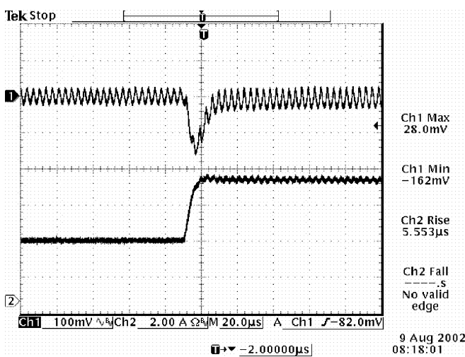
V_{out}=1.8\text{V} 50% to 100% load transients at 3.3V input and T_a=25^\circ\text{C}
